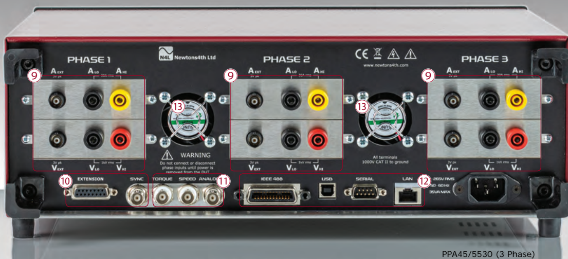
PPA45/5530 (3 Phase)
