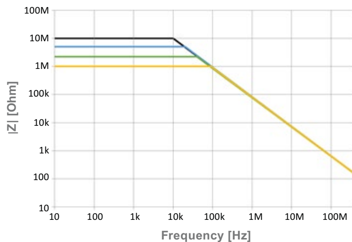
Typical Differential Input Impedance BumbleBee® Series
