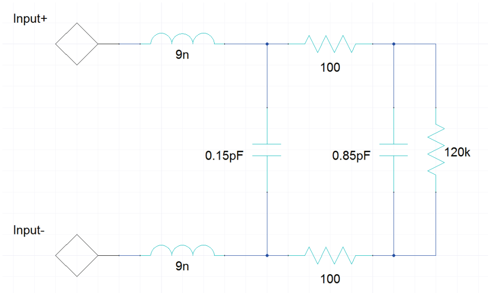
ZDxxxx Differential Input Equivalent Circuit
